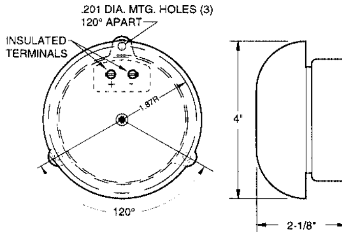
Detail: Model 2464012060
